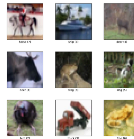
CIFAR-10
