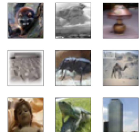
CIFAR-100
